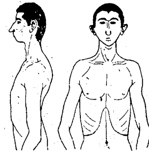
Den leptosome type.
